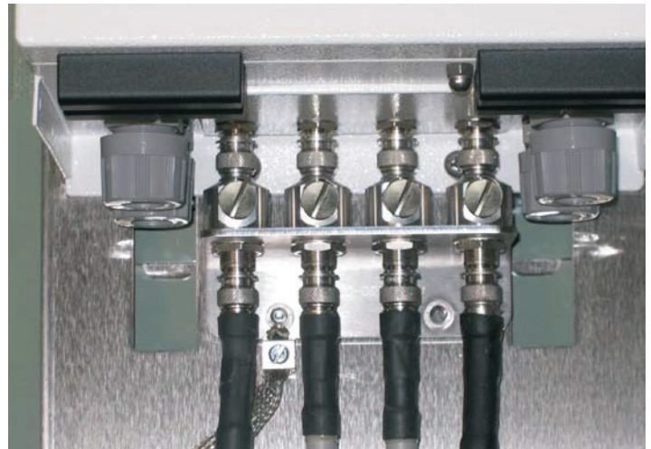
Example installation of lightning supression kit on a OmniTrax processor
