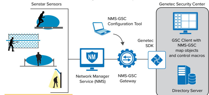
NMS-GSC system integration
