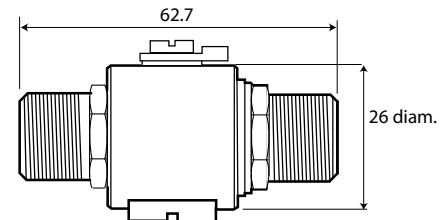
Lightning arrestor
