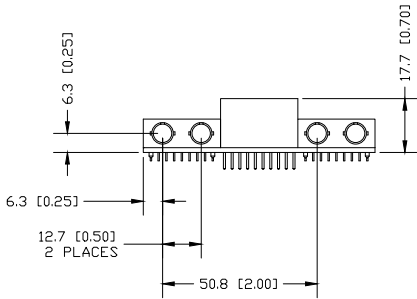
SILVER G2 COMM CARD SMFO, 00BA2101-001 SCALE 1 : 1
