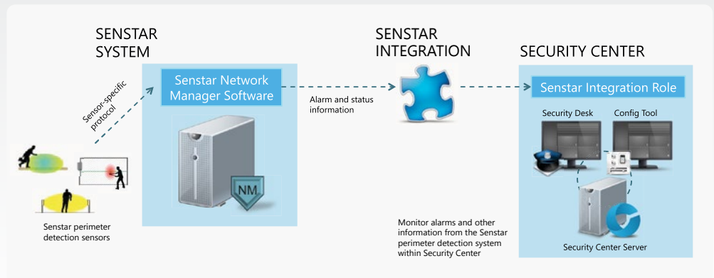
Senstar® Integration with Security Center
