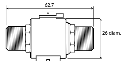
Lightning arrester
